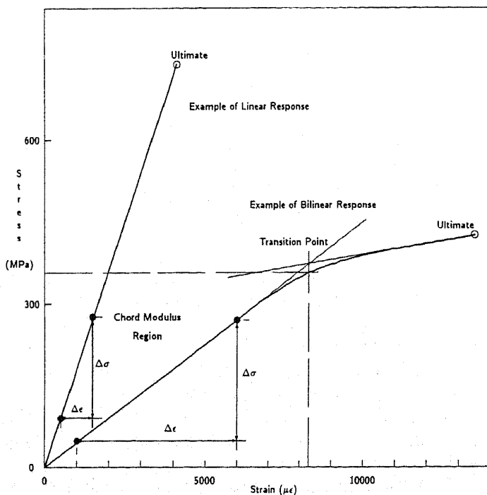
FIG. 5 Typical Tensile Stress-Strain Curves
